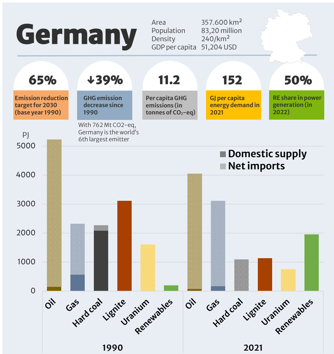
Figure 1: Germany – energy facts and energy balance
